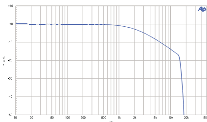
Figure 16. FIL-D75F. 75\ \mu\text{s} with 19 kHz (FM) notch De-emphasis Filter.
