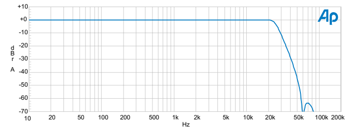
Figure 25. Typical response of 20 kHz “pre-analyzer” filter.
