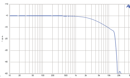
Figure 13. FIL-D50F. 50\ \mu\text{s} with 19 kHz (FM) notch De-emphasis Filter.
