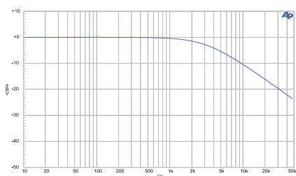
Figure 12. FIL-D50. 50\ \mu\text{s} De-emphasis Filter.
