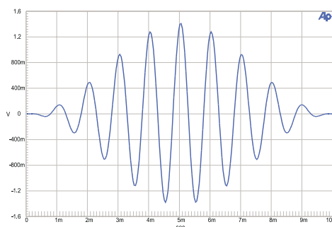
Figure 30. Shaped Sine Burst signal. (1 kHz, 10 cycles)
