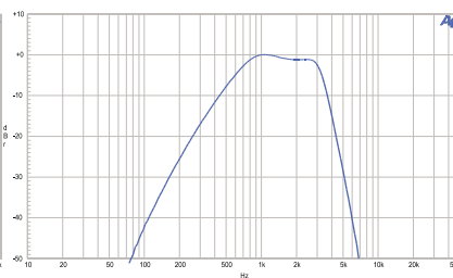
Figure 10. FIL-CMS. C-Message Weighting Filter (ANSI/IEEE 743-1984)
