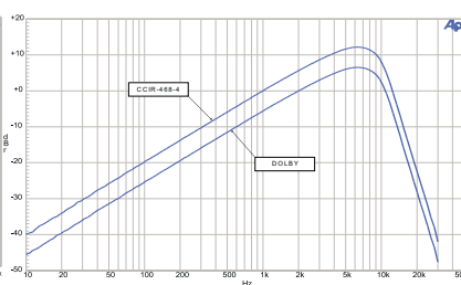
Figure 8. FIL-CCR. IEC468 (CCIR)/ DIN 45404 Noise Weighting Filter
