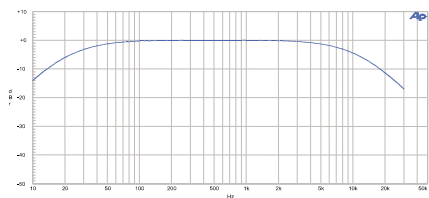
Figure 11. FIL-CWT. "C" Weighting (IEC-179)
