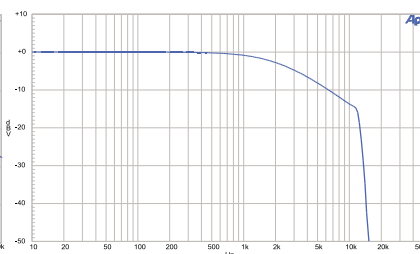
Figure 15. FIL-D75B. 75\ \mu\text{s} with 15.734 kHz (NTSC) notch De-emphasis Filter
