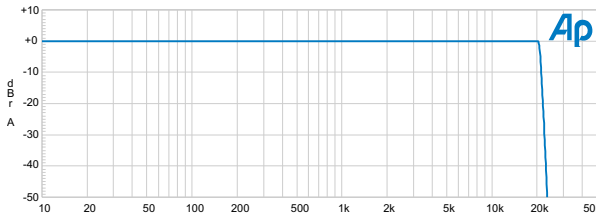
Figure 17. FLP-B20K “Brick Wall” 20 kHz low pass filter. Complies with requirements of AES17 for D/A converter THD+N measurements.
