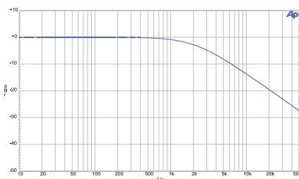
Figure 14. FIL-D75. 75\ \mu\text{s} De-emphasis Filter.
